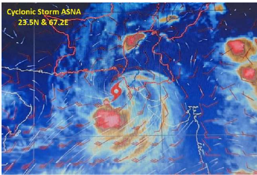
Satellite image (30 August 2024, 2130 PST)
