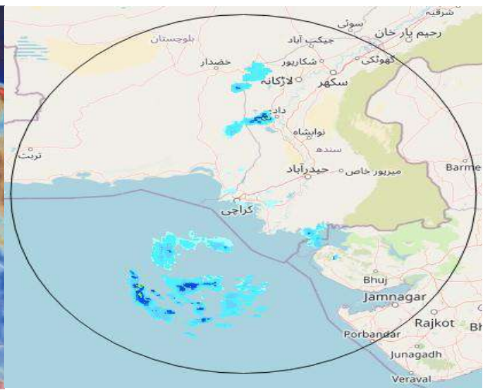
PMD Radar Image August 30, 2024 2130PST
