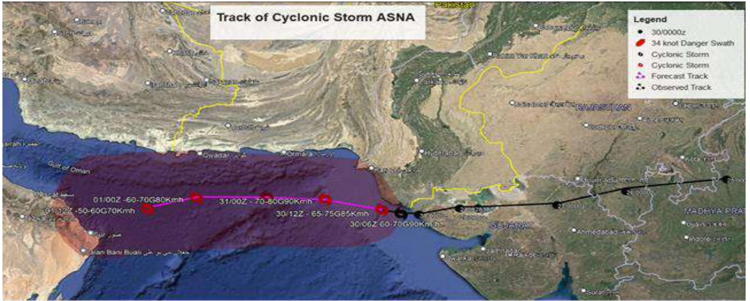
Observed & Forecast Track
